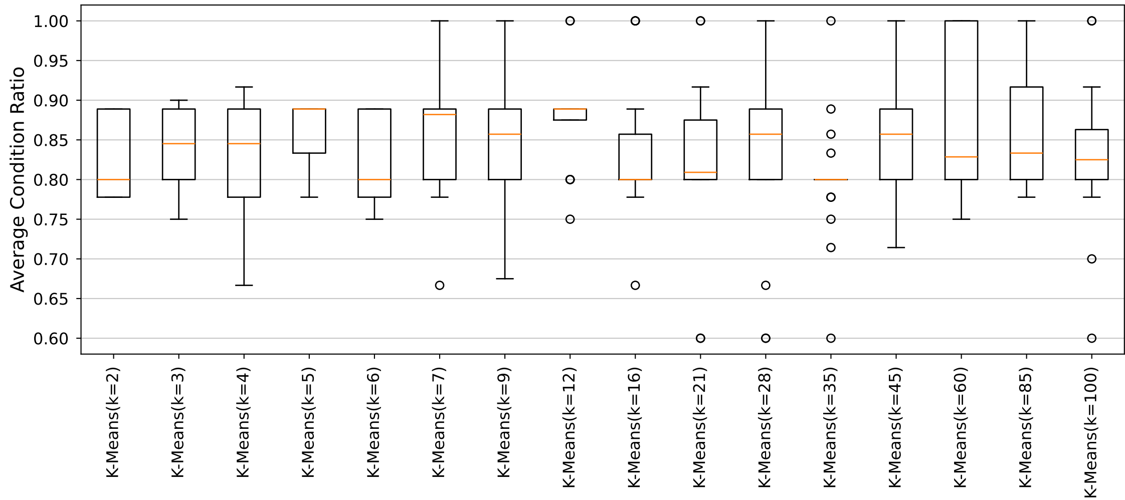
YARA Rules Average Condition Ratio Distribution (Cluster2_Size100 dataset)
